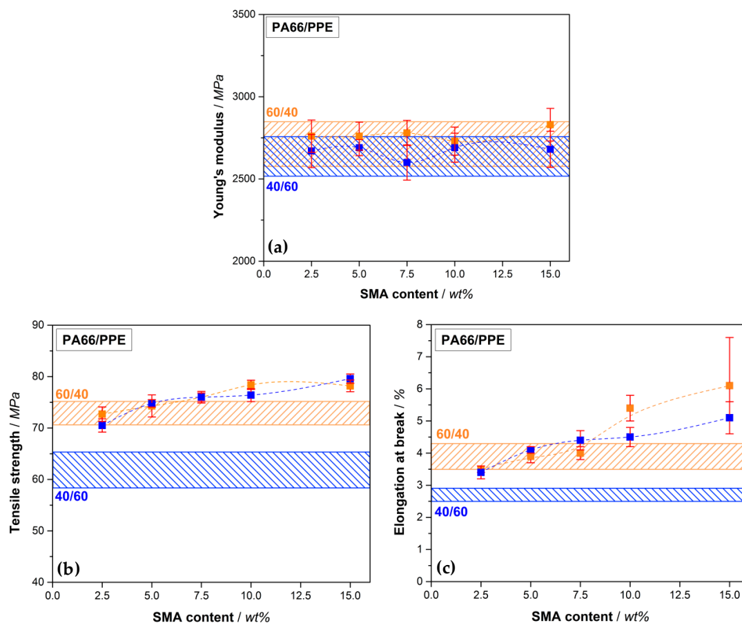
Figure 5. Tensile properties of PA66/PPE/SMA ternary blends with Young's modulus (a), tensile strength (b) and elongation at break (c), depending on the SMA content, with 60/40 blend ratio (orange rectangular) and 40/60 blend ratio (blue rectangular). Orange (60/40) and blue bars (40/60) stand for the PA66/PPE binary blend values without SMA.
