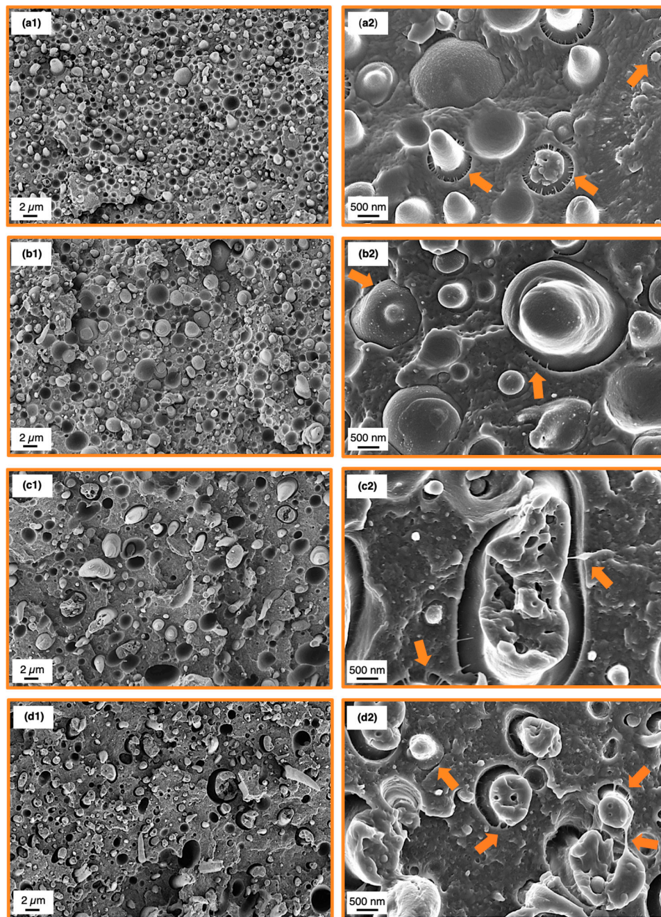
Figure 6. Scanning electron microscopy (SEM) micrographs subsequent to tensile testing of the 60/40 binary blend ( a1 ), 5 wt% SMA ( b1 ), 10 wt% SMA ( c1 ) and 15 wt% SMA ( d1 ). Higher magnifications of the corresponding blends are depicted at the right column ( a2 , b2 , c2 , d2 ). Orange arrows indicate matrix fibrillations.
